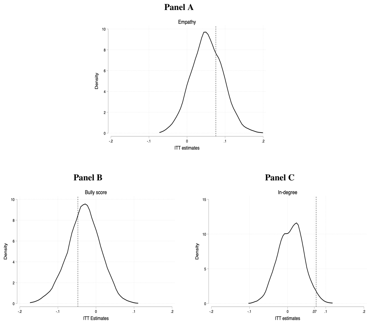
Figure I4: Model Validation
