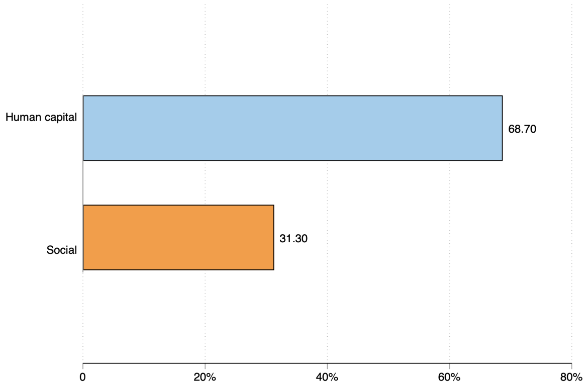
Figure 2: Decomposition Results
